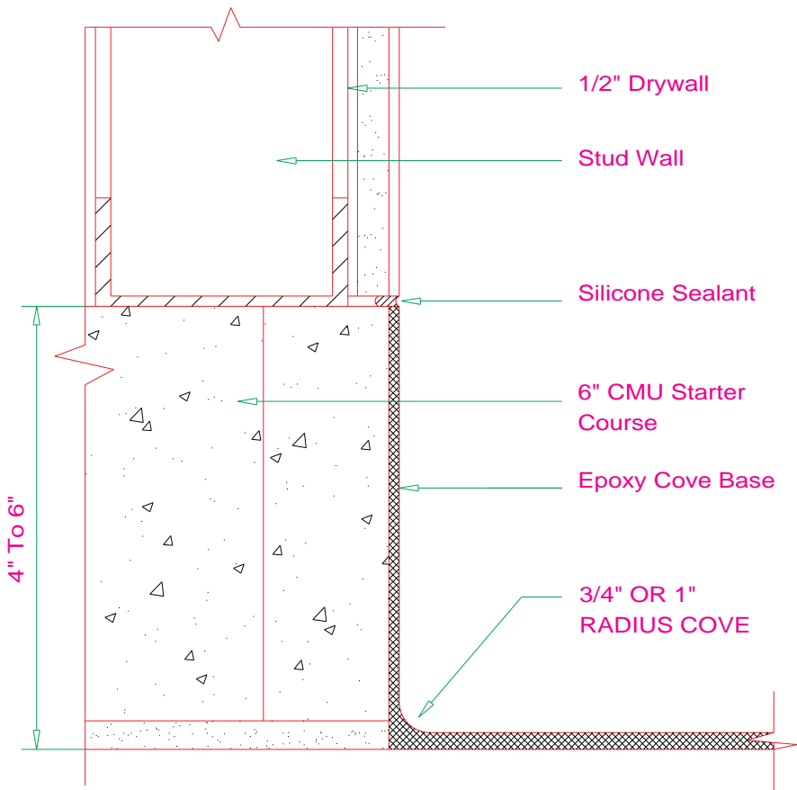
Cove Base Termination In Block Joint
