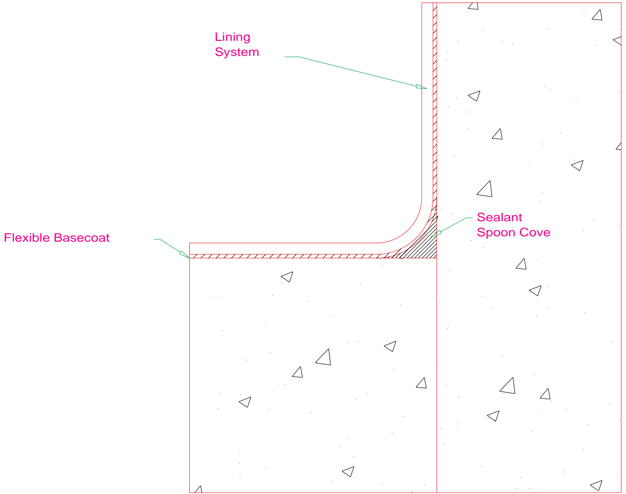
Cove Butt Joint
